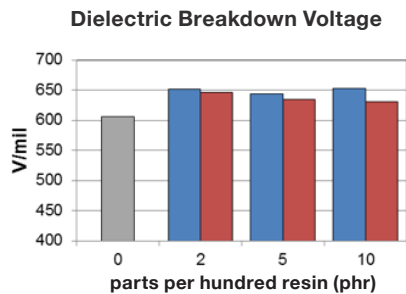
Figure 1: Dielectric breakdown voltage (ASTM D149-13, method A, AC 2000 V/s)
